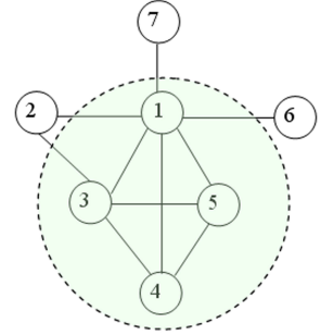
Figure 1: An example of mining a local clique from a local neighborhood graph.
